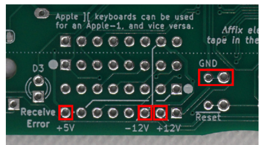
Points to check for shorts (back side PCB).
