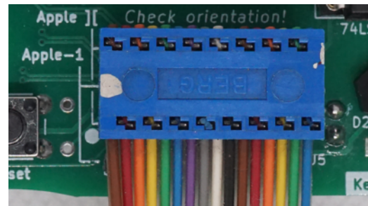
Apple ][ keyboards connect the other way around, pin-1 pointing to the left (J6 + J8).
