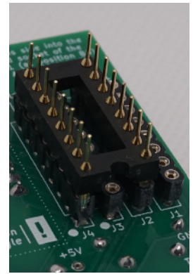
Adapter positioned for the Apple ][ .
