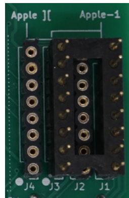
Position of adapter for Apple-1 usage.
