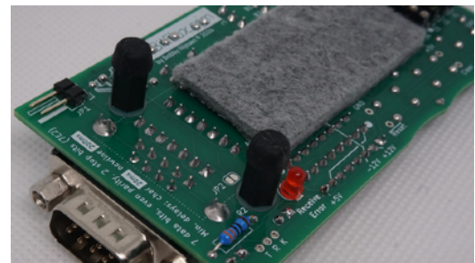
Mounting of the standoffs with caps and washers. Keep JP2 clear when affixing the felt.
